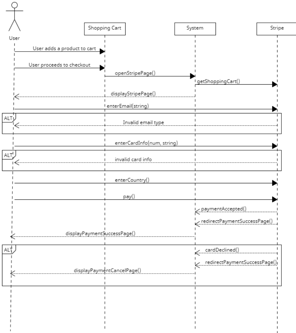
Figure 4: Payment Sequence Diagram
