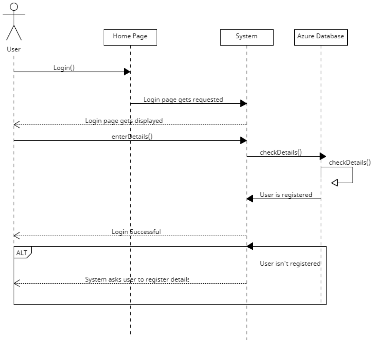
Figure 2: Login Sequence Diagram
