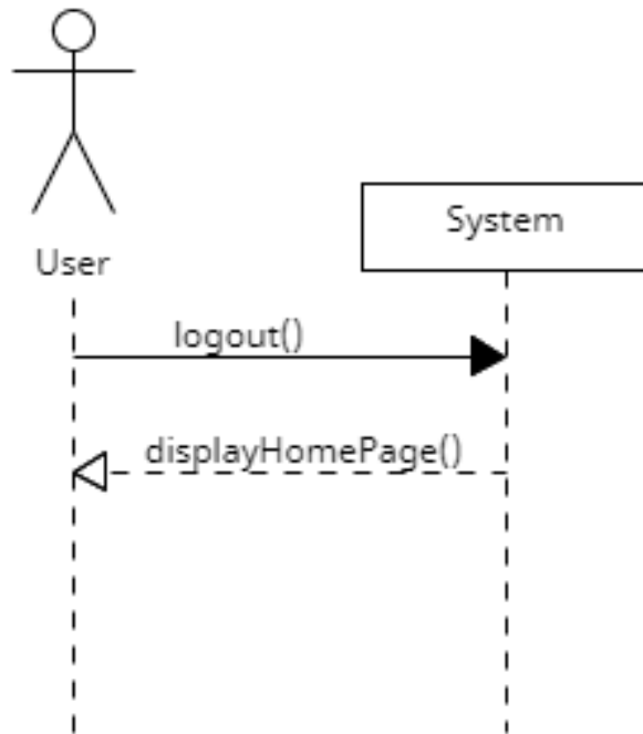
Figure 3: Logout Sequence Diagram
