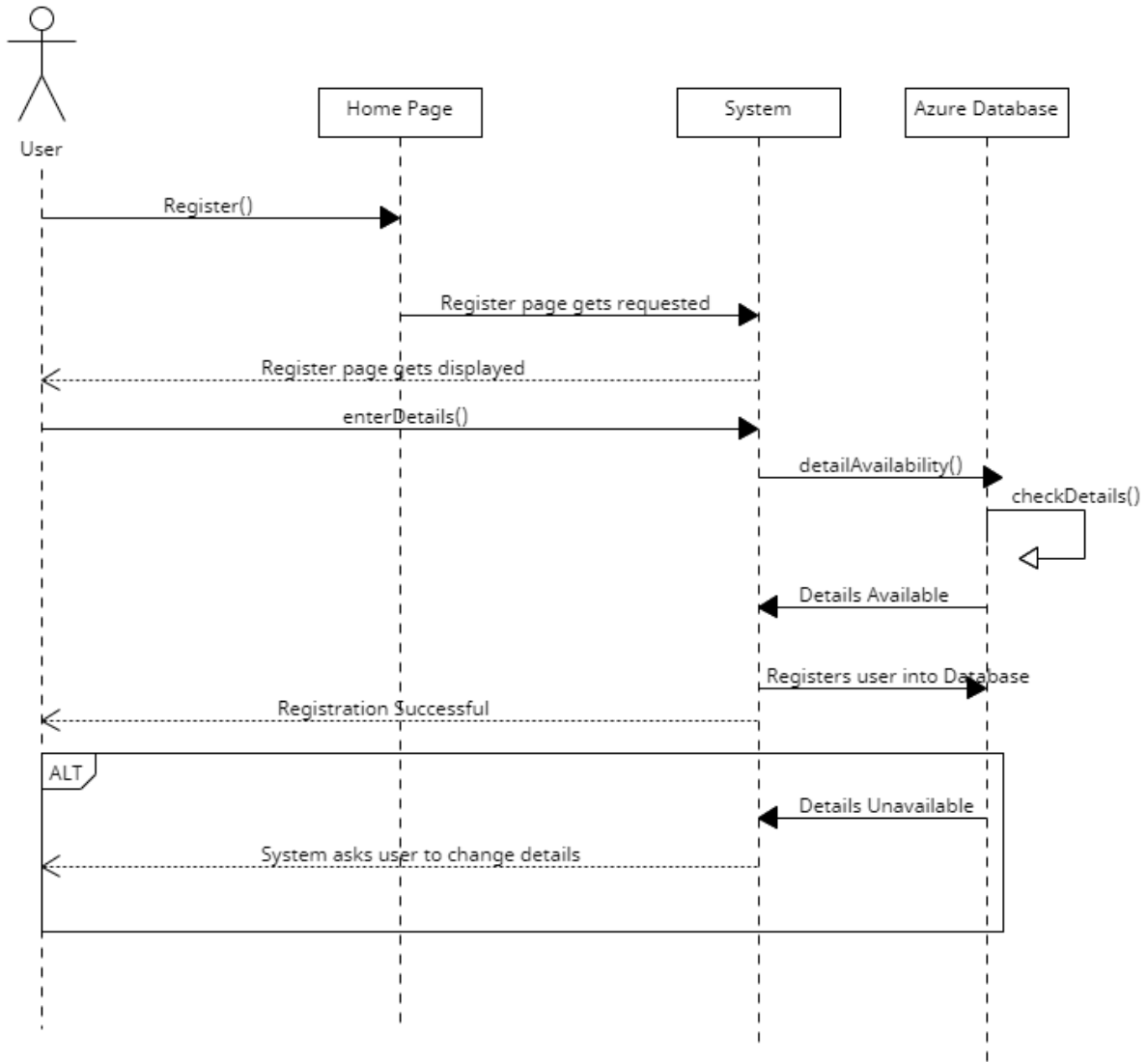
Figure 1: Register Sequence Diagram
